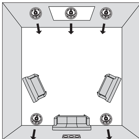
Home Theater Example #2 (diffuse surround effects)
