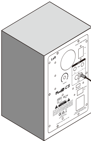
RCA Unbalanced Connection
