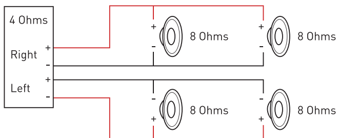
Parallel Speaker Wire Diagram
